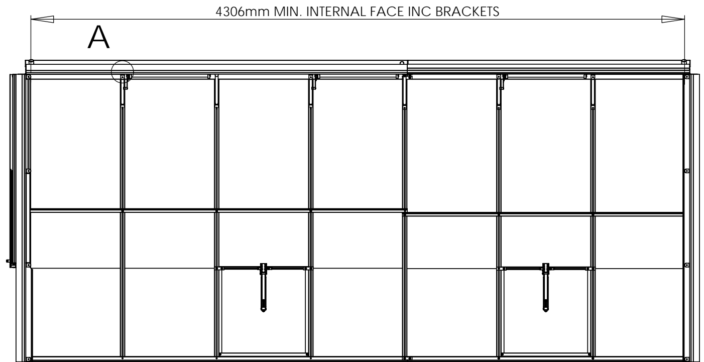
6LT x 14' WALL PLAN
